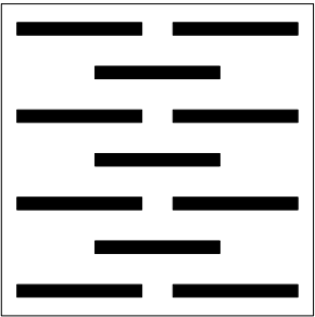
Type :Diagonal Slotted Hole Size :6 ×60mm C/C :21 ×75mm
